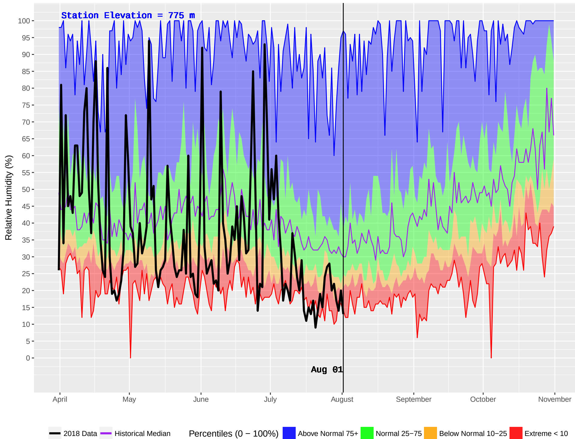
ELKO (412) : Historical (1970–2016) and Current (2018) Daily Relative Humidity
